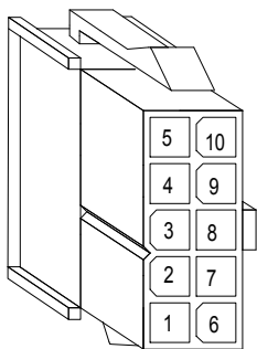
Molex 39-01-2101
